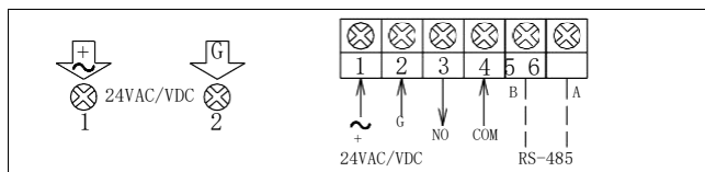
F2000TSM-VOC-L101C TSM-VOC-L110C-(C)
