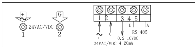
F2000TSM-VOC-S110C/S100C TSM-VOC-L110C/L100C
